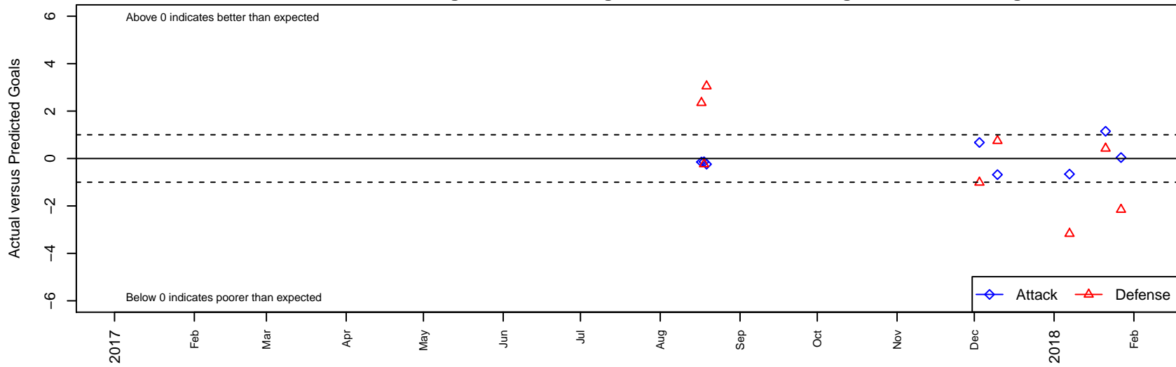
GS Surf C G02 Dots are actual minus expected GF (blue circles) and GA (red triangles). Blue line is smoothed change in attack strength. Red is smoothed change in defense strength.
